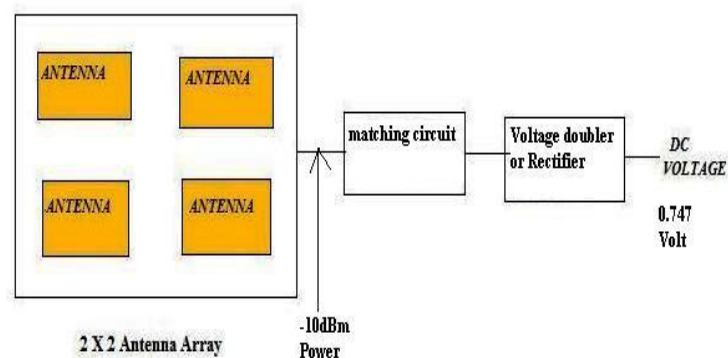
Figure 1: Block diagram of energy harvesting system
