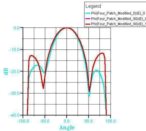
Figure 4: 2D cut out of radiation pattern in phi-plane in fourth
