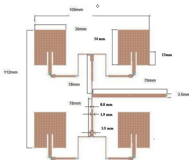
Figure 2: (2x2) Microstrip rectangular patch antenna array
