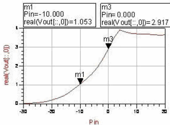
Figure 9: Simulated value of P_{in} Vs V_{out} in open circuit
