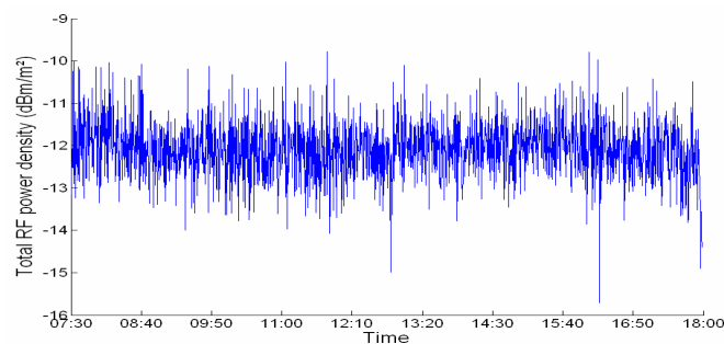
Fig.3 Measured RF power density versus time (680MHz-3500MHz)
