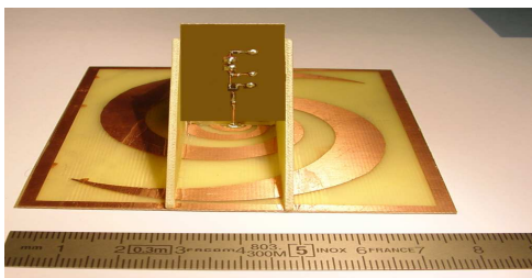
Fig.15 Rectenna prototype
