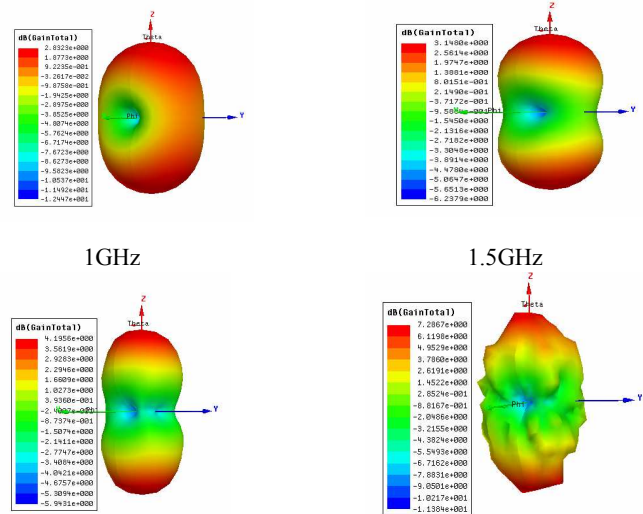
Fig. 12: Radiation pattern of spiral antenna.
